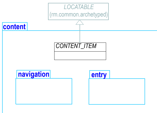
FIGURE 14 rm.composition.content package
