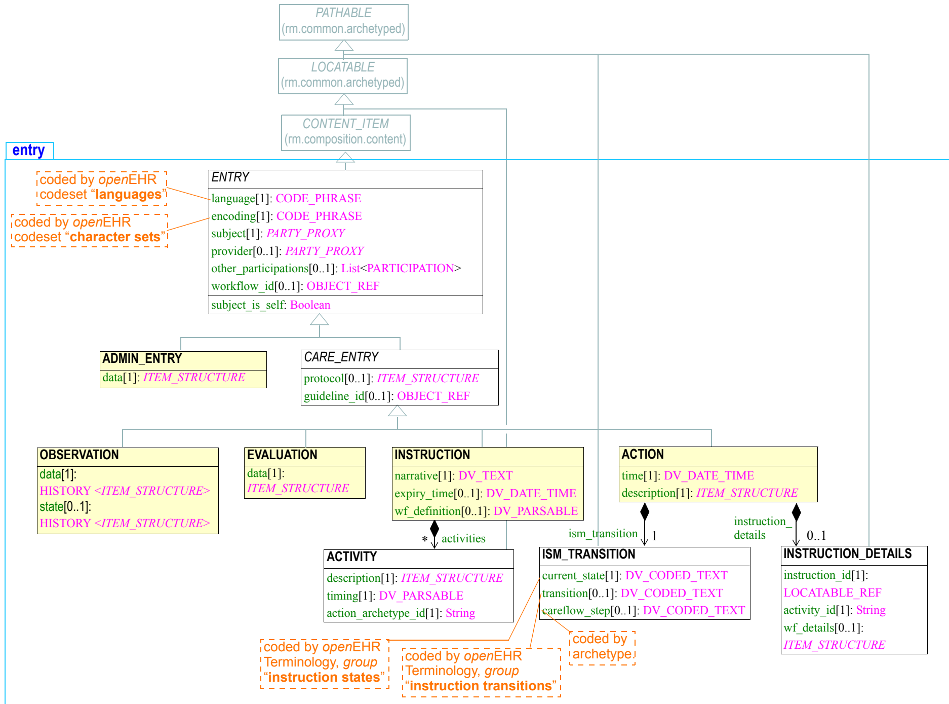
FIGURE 20 rm.composition.content.entry Package
