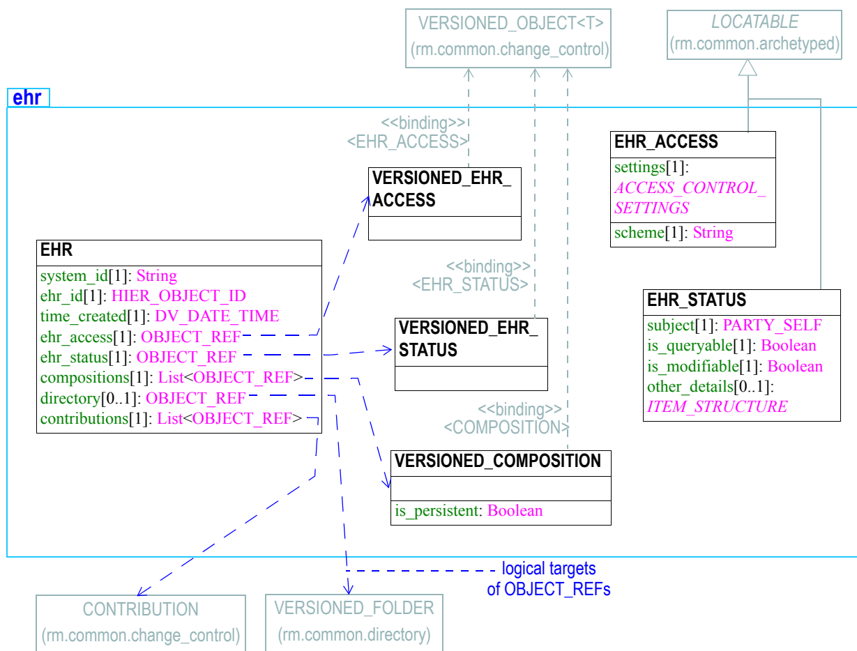
FIGURE 4 rm.ehr Package
